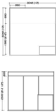
TYPICAL 10' X 10' BOOTH CW COUNTER
